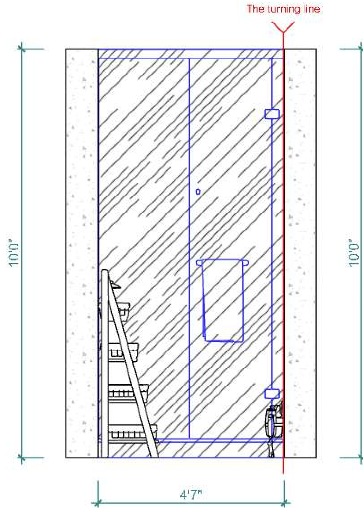
Bathroom Elevation B(3/5"=1'-0")
