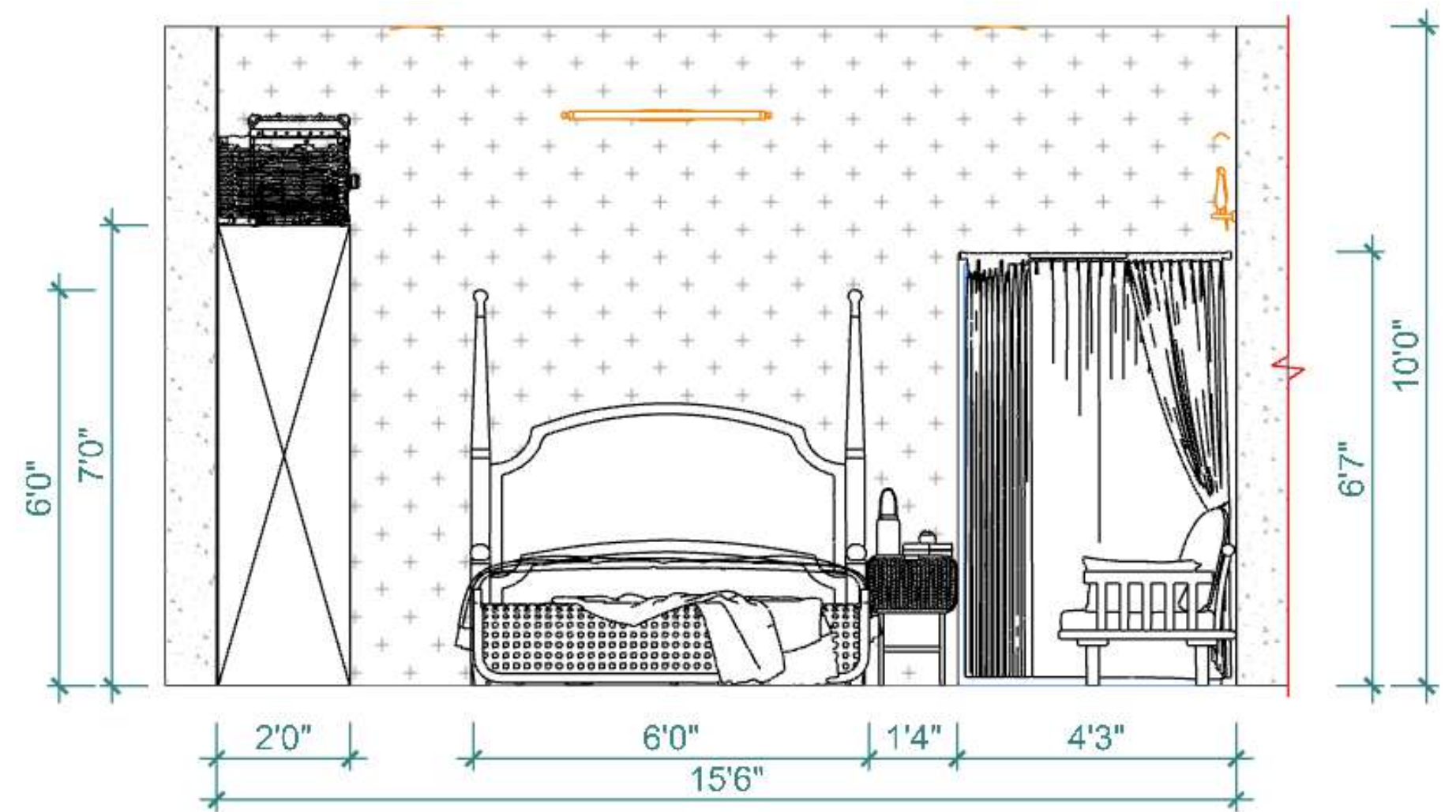
Bedroom Elevation B(1/2"=1'-0")
