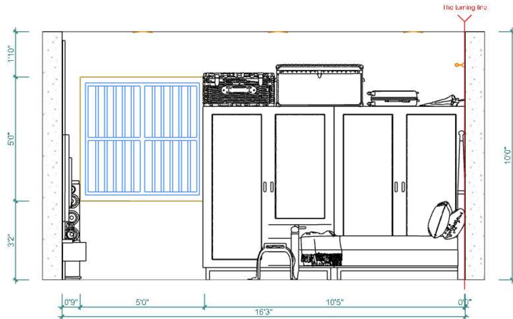
Bedroom Elevation A(1/2"=1'-0")
