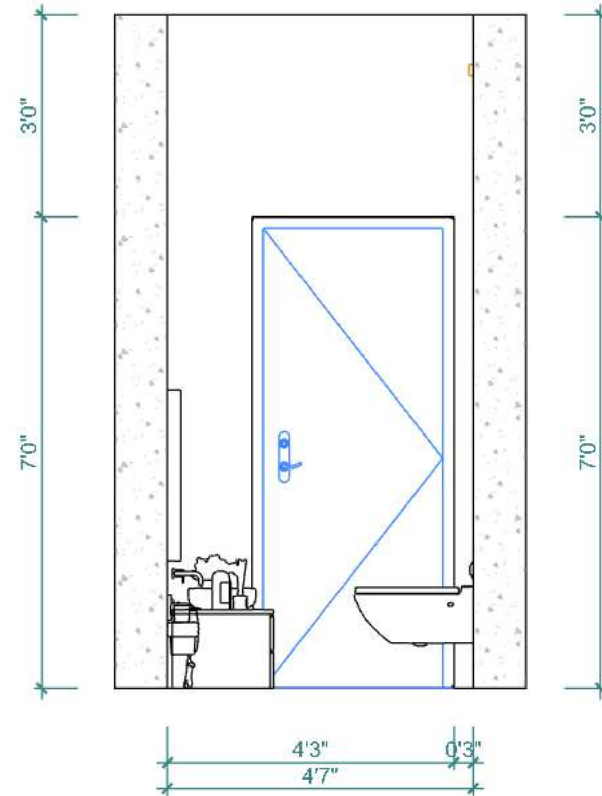
Bathroom Elevation D(2/3"=1'-0")
