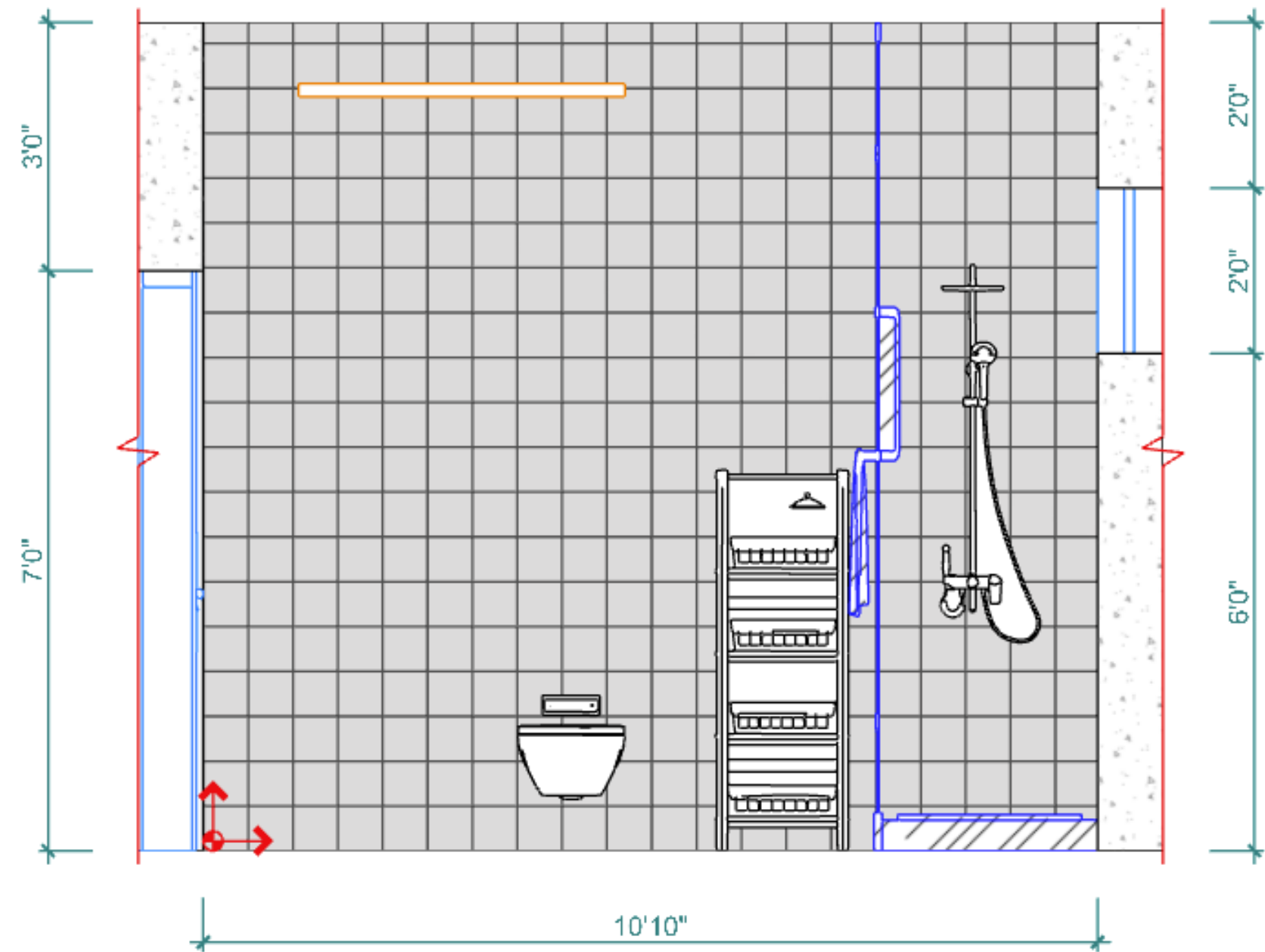
Bathroom Elevation A(3/5"=1'-0")
