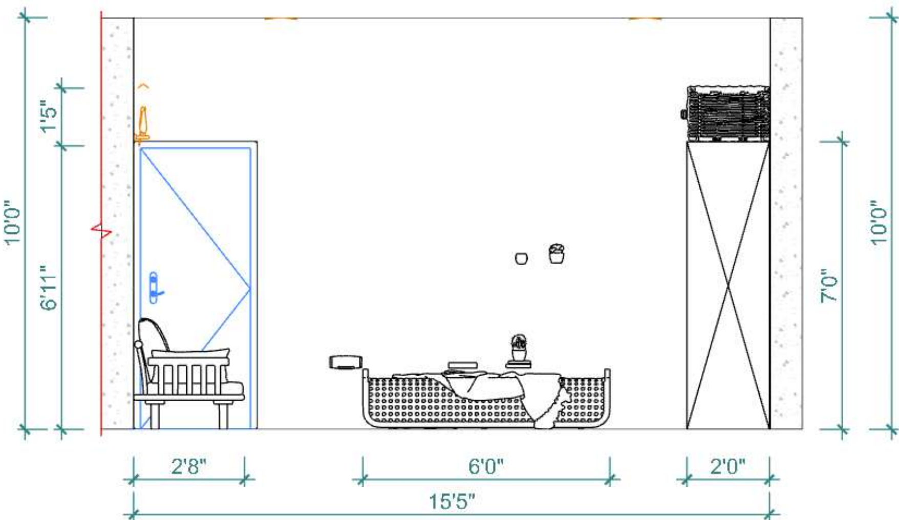
Bedroom Elevation D(1/2"=1'-0")
