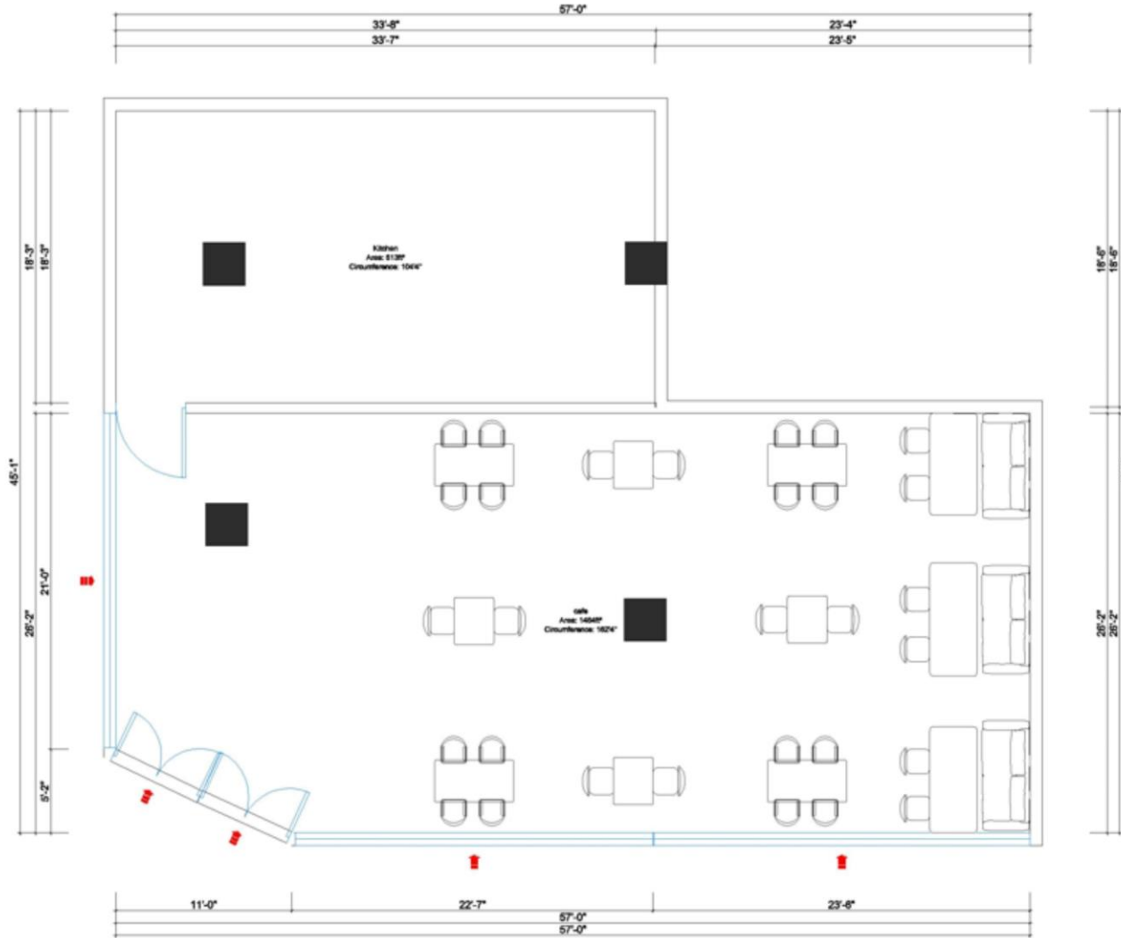
Furniture Plan(12/95"=1'-0")
